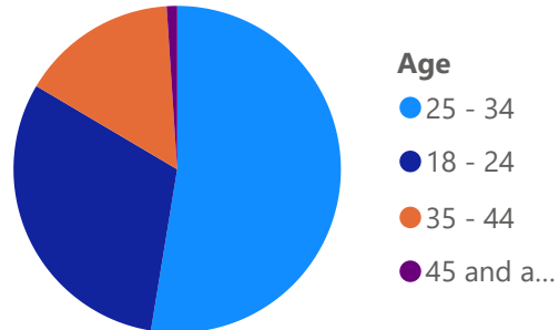
Age
